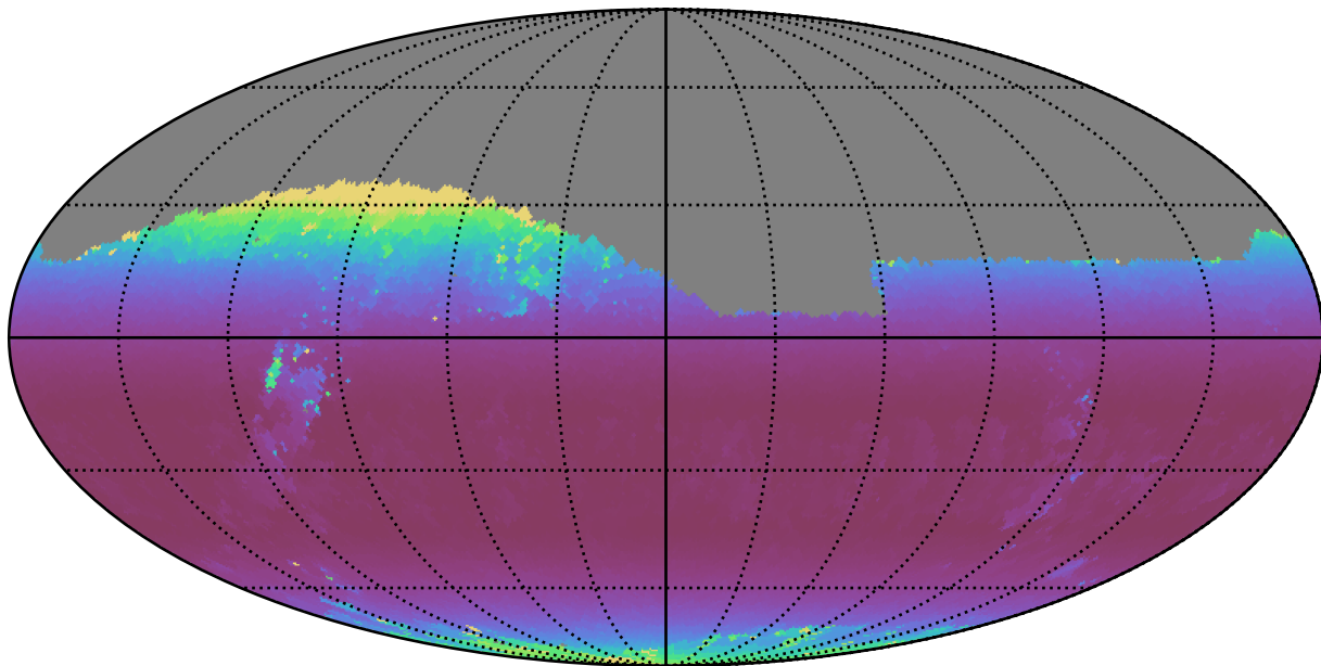
weather_cloudso1v3.4_10yrs Yr 1 z band: Min airmass
