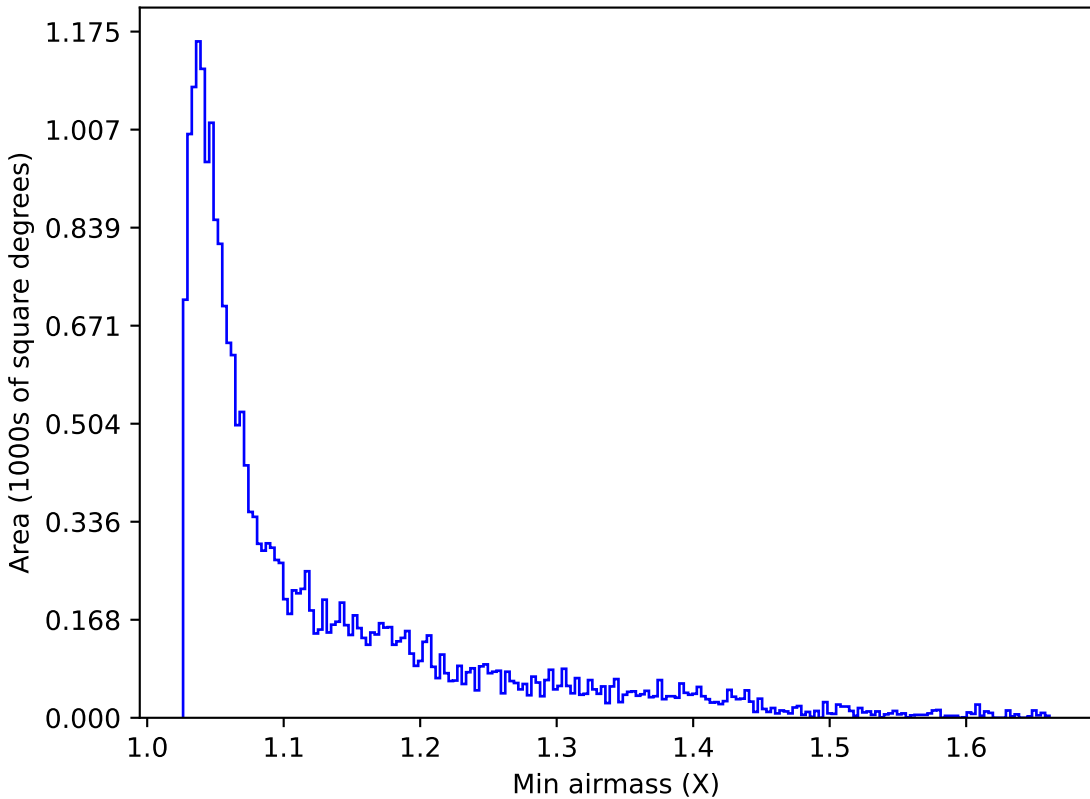
weather_cloudso1v3.4_10yrs Yr 1 y band: Min airmass
