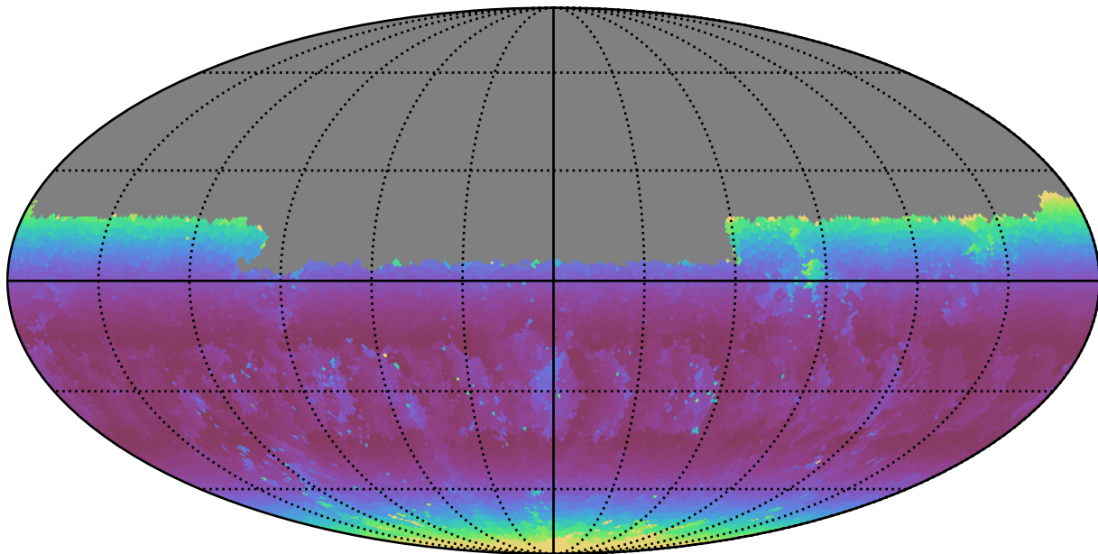
weather_cloudso1v3.4_10yrs Yr 1 u band: Min airmass
