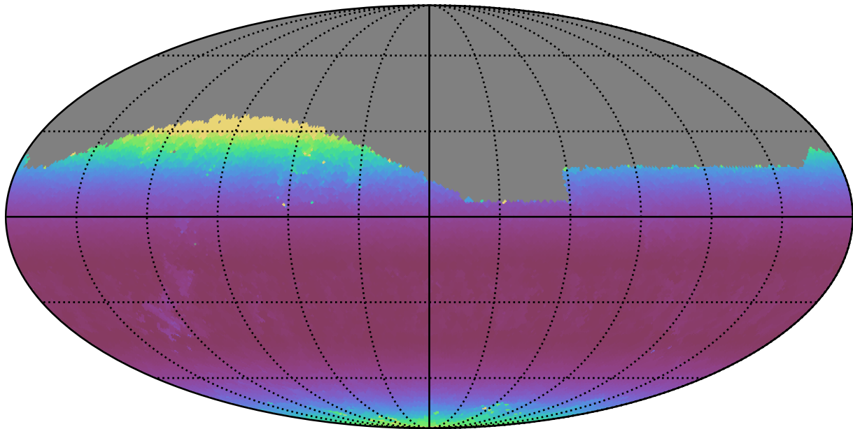
weather_cloudso1v3.4_10yrs Yr 1 r band: Min airmass
