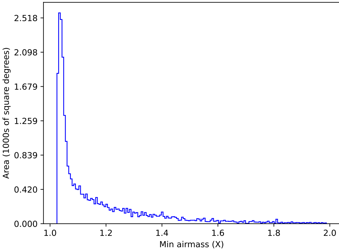
weather_cloudso1v3.4_10yrs Yr 1 r band: Min airmass
