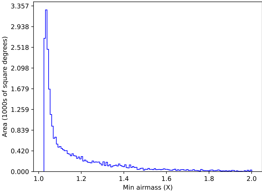
weather_cloudso1v3.4_10yrs Yr 1 i band: Min airmass
