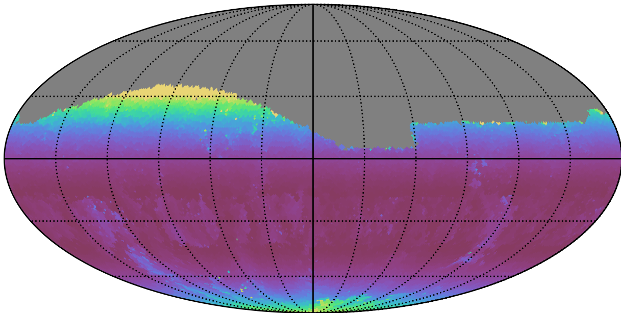
weather_cloudso1v3.4_10yrs Yr 1 g band: Min airmass
