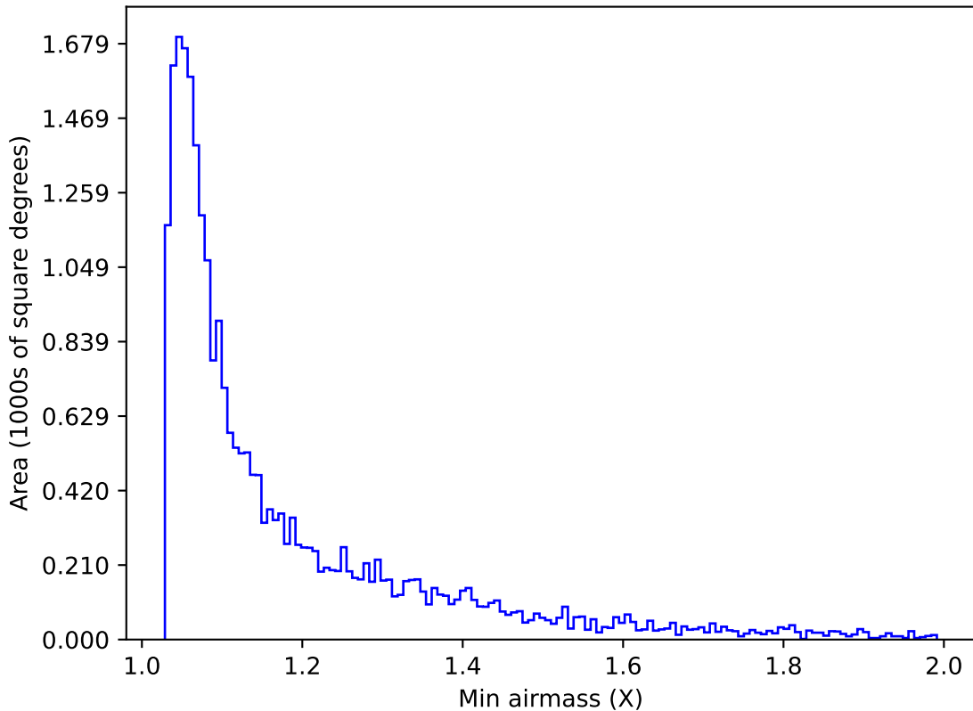
weather_cloudso1v3.4_10yrs Yr 1 g band: Min airmass
