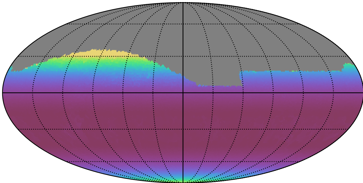
weather_cloudso1v3.4_10yrs Yr 1 all bands: Min airmass
