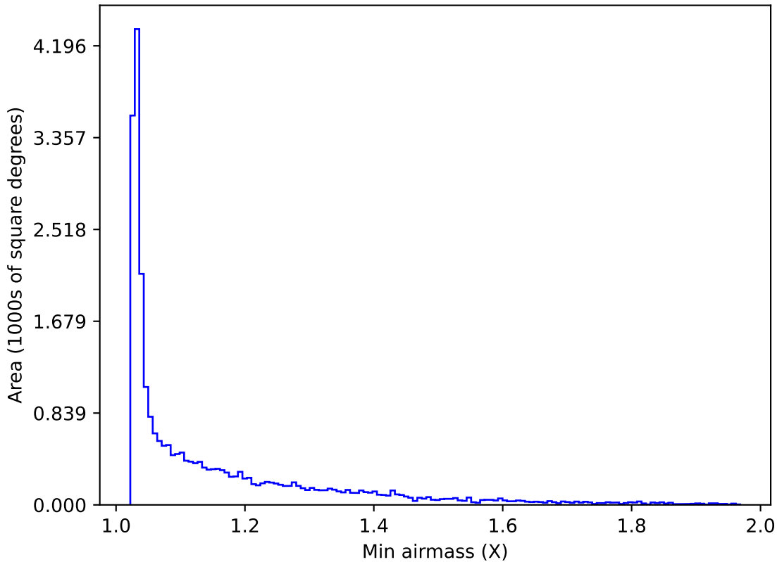
weather_cloudso1v3.4_10yrs Yr 1 all bands: Min airmass
