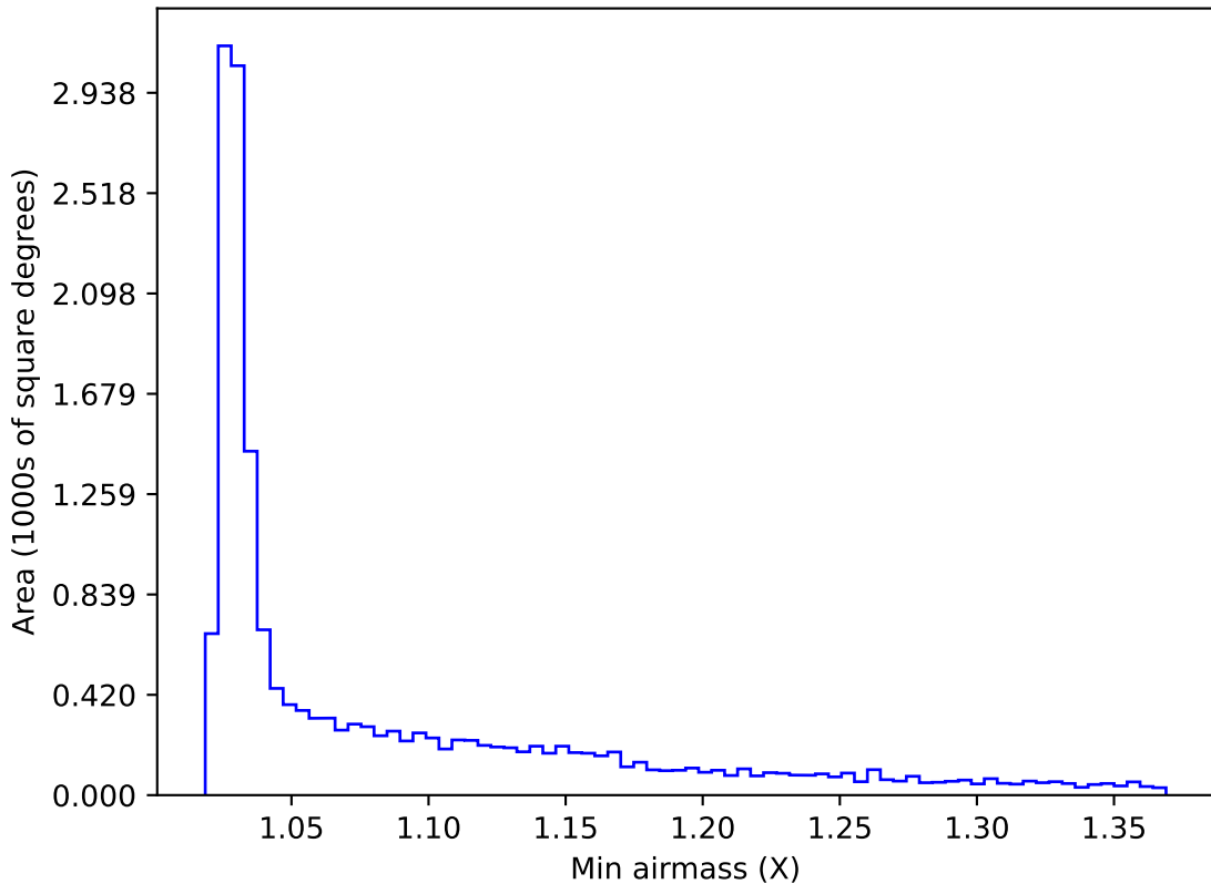
weather_cloudso1v3.4_10yrs WFD z band: Min airmass
