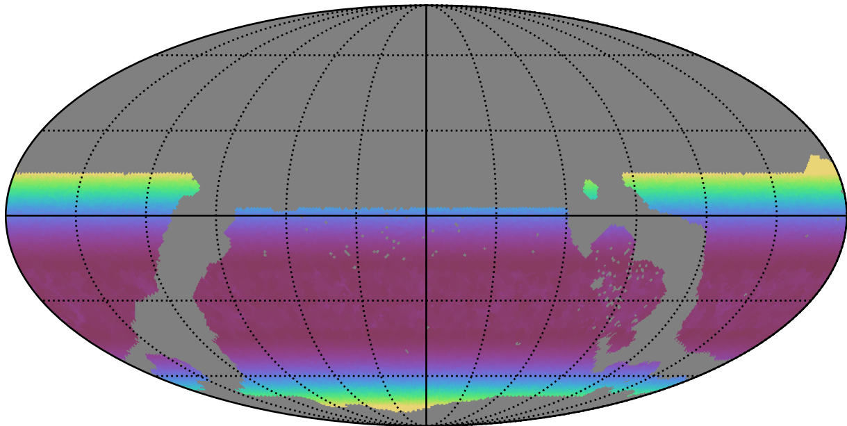
weather_cloudso1v3.4_10yrs WFD y band: Min airmass
