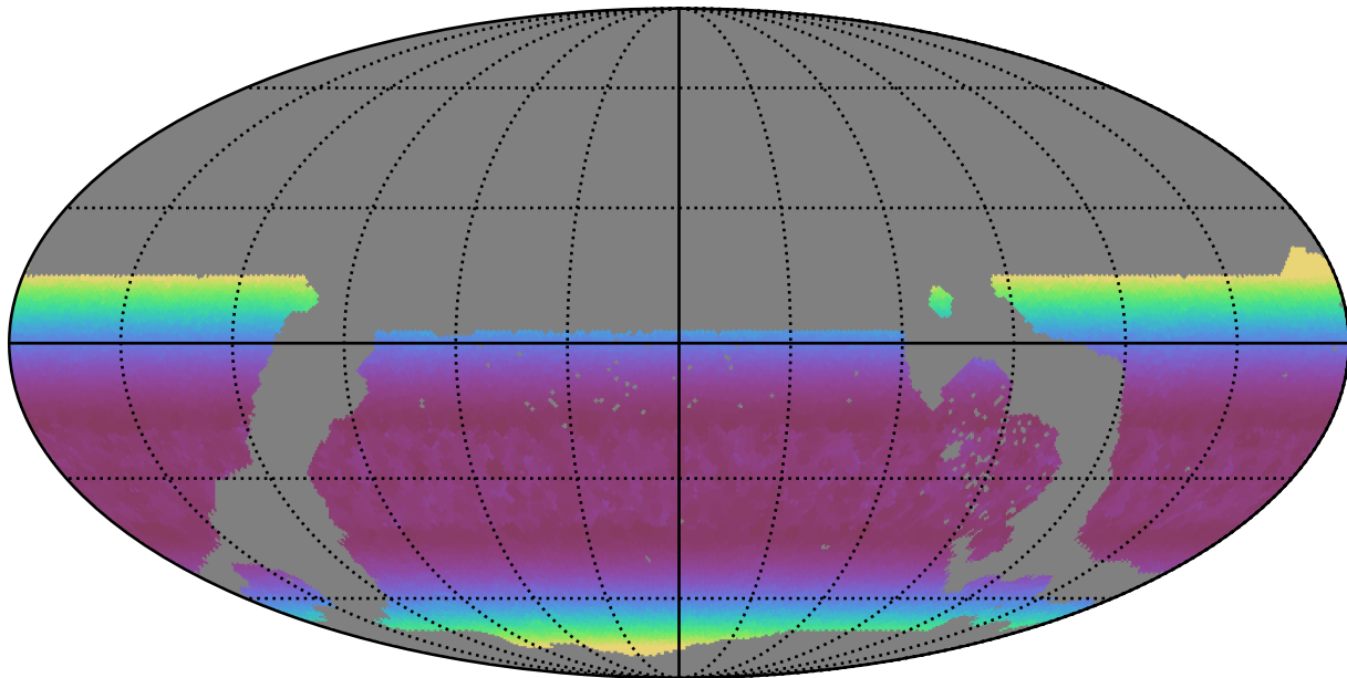
weather_cloudso1v3.4_10yrs WFD u band: Min airmass
