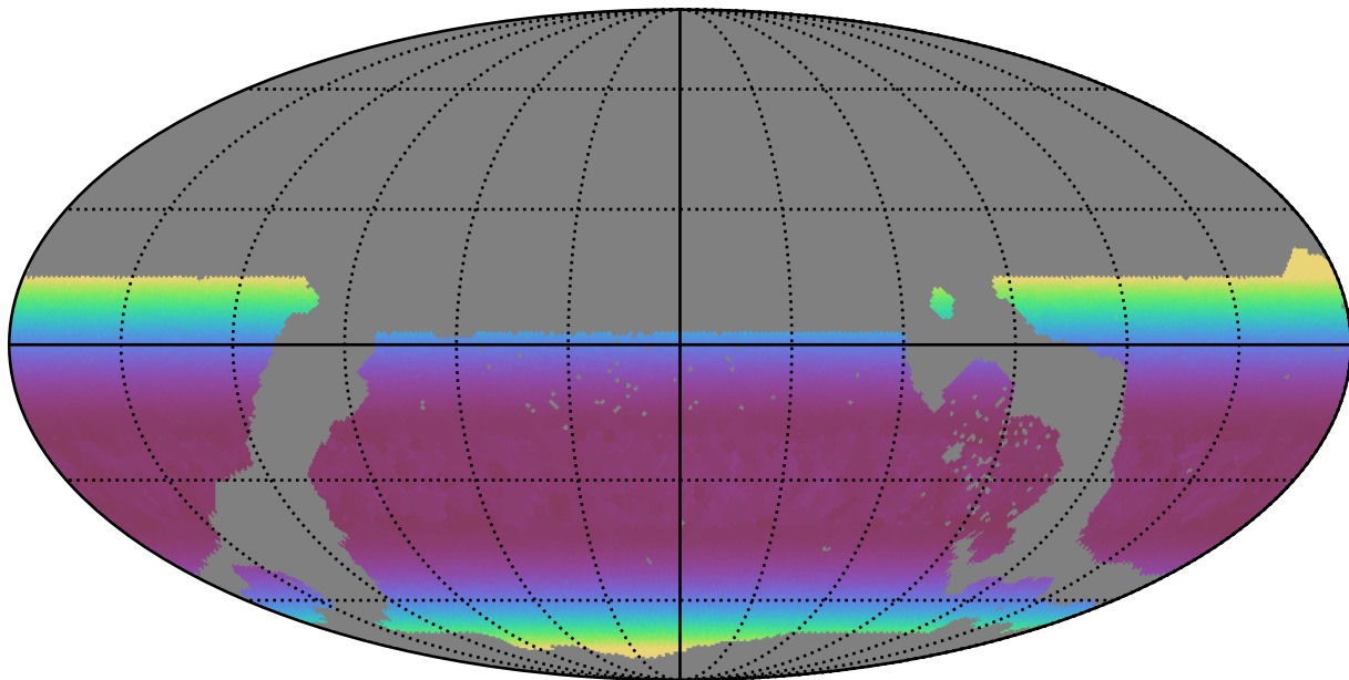
weather_cloudso1v3.4_10yrs WFD r band: Min airmass
