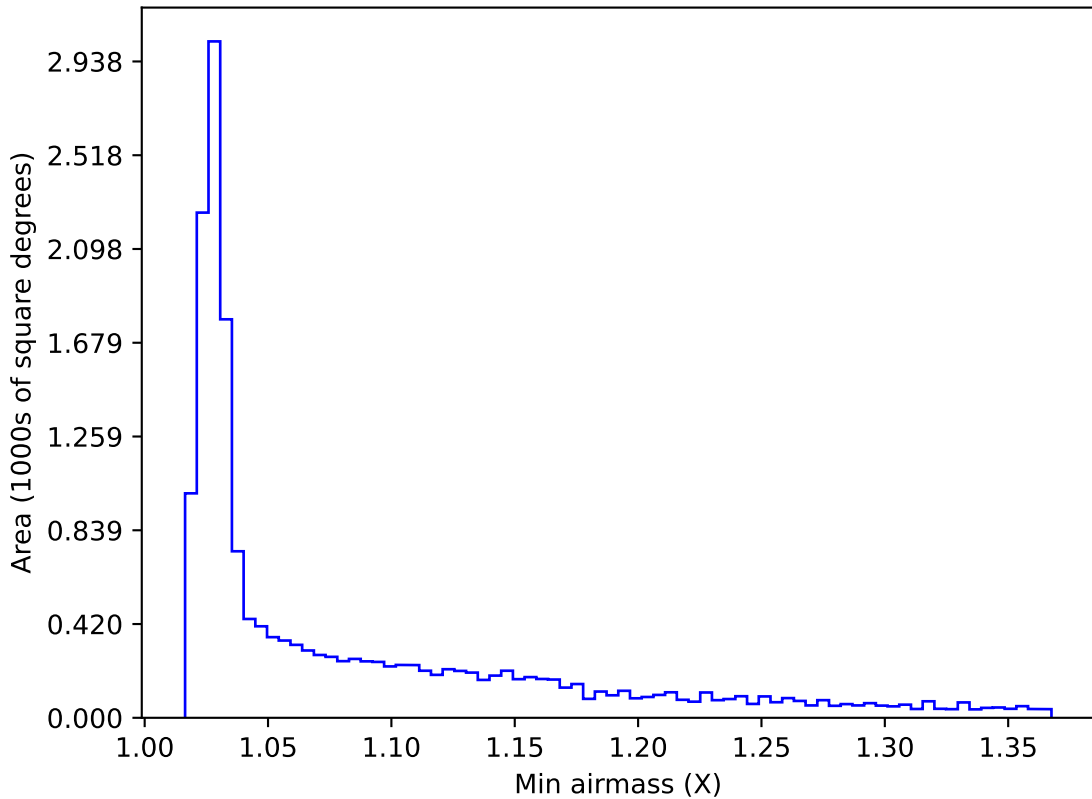
weather_cloudso1v3.4_10yrs WFD r band: Min airmass
