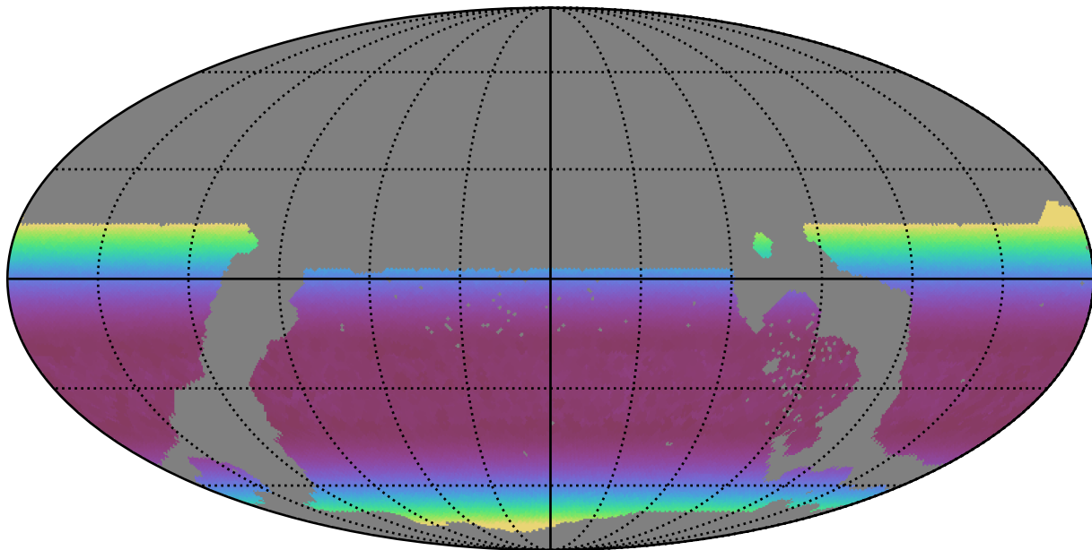
weather_cloudso1v3.4_10yrs WFD i band: Min airmass
