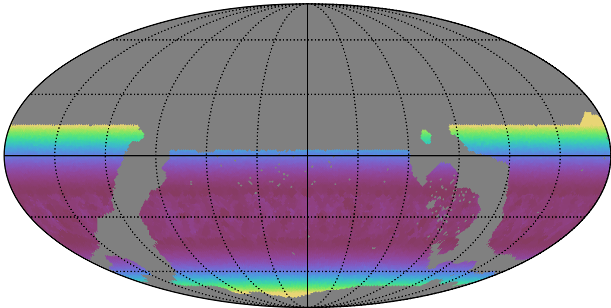
weather_cloudso1v3.4_10yrs WFD g band: Min airmass
