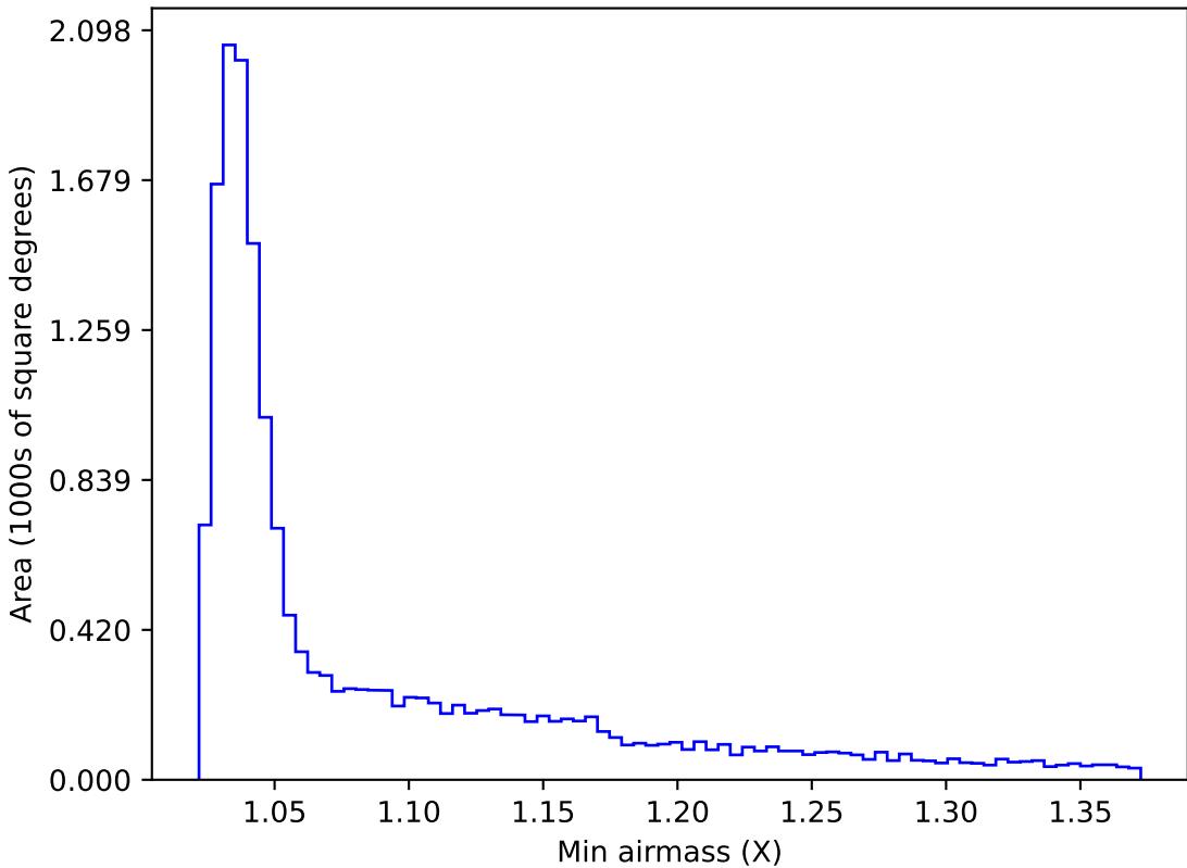
weather_cloudso1v3.4_10yrs WFD g band: Min airmass
