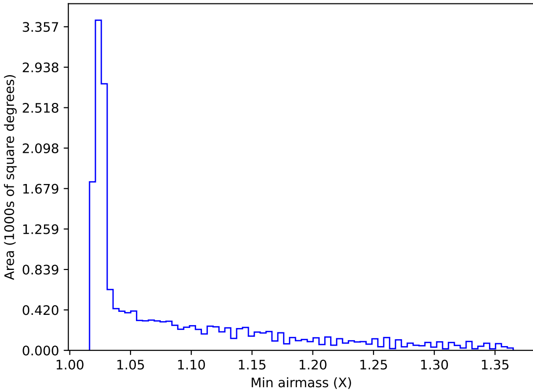
weather_cloudso1v3.4_10yrs WFD all bands: Min airmass
