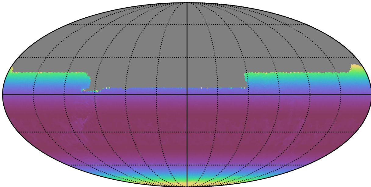
weather_cloudso1v3.4_10yrs All sky y band: Min airmass
