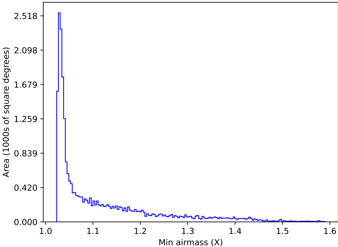
weather_cloudso1v3.4_10yrs All sky y band: Min airmass
