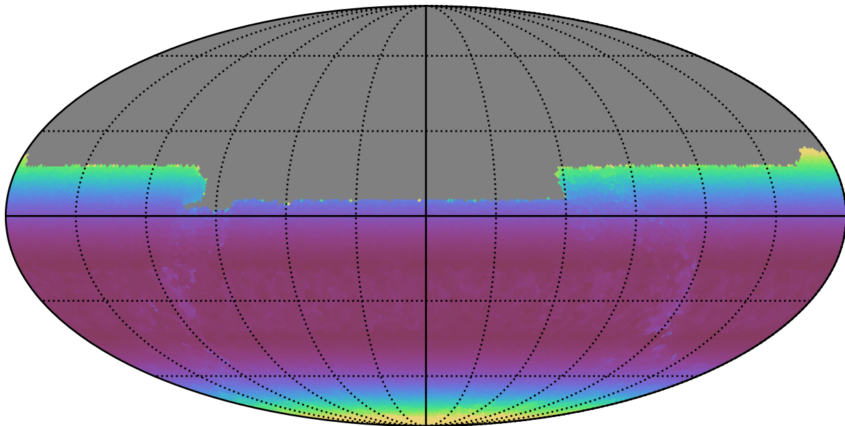
weather_cloudso1v3.4_10yrs All sky u band: Min airmass
