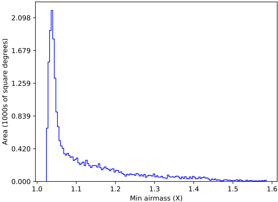
weather_cloudso1v3.4_10yrs All sky u band: Min airmass
