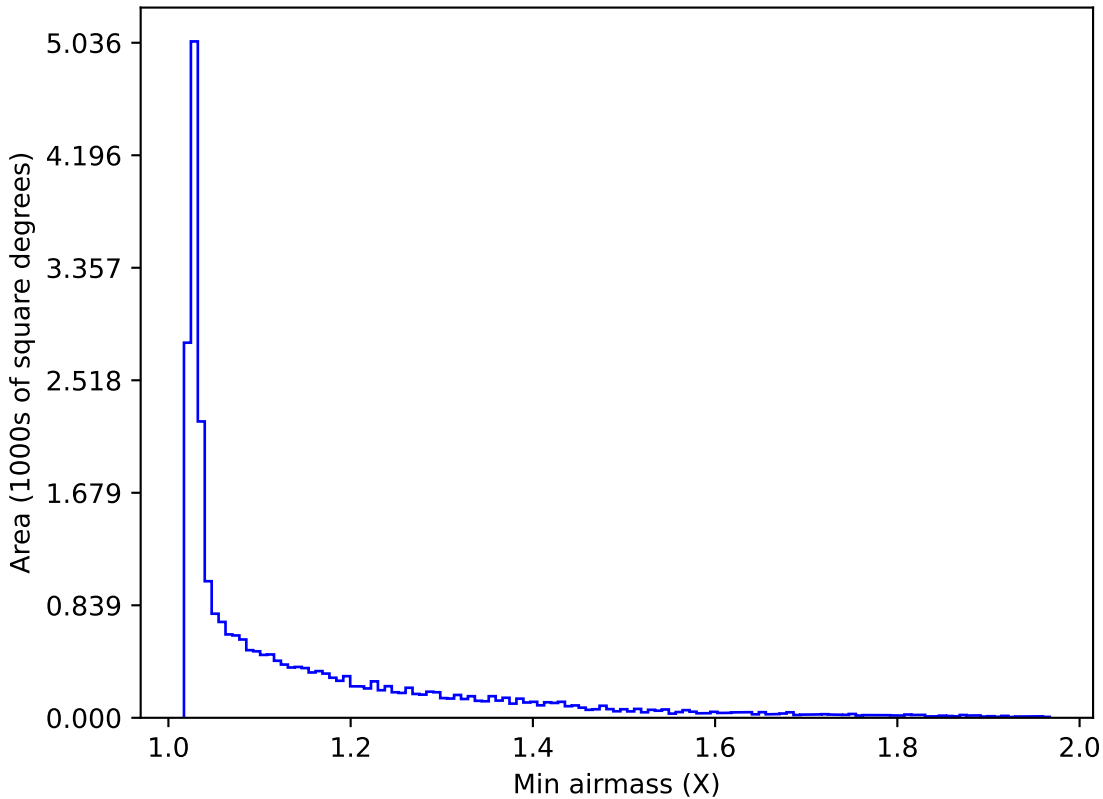
weather_cloudso1v3.4_10yrs All sky r band: Min airmass
