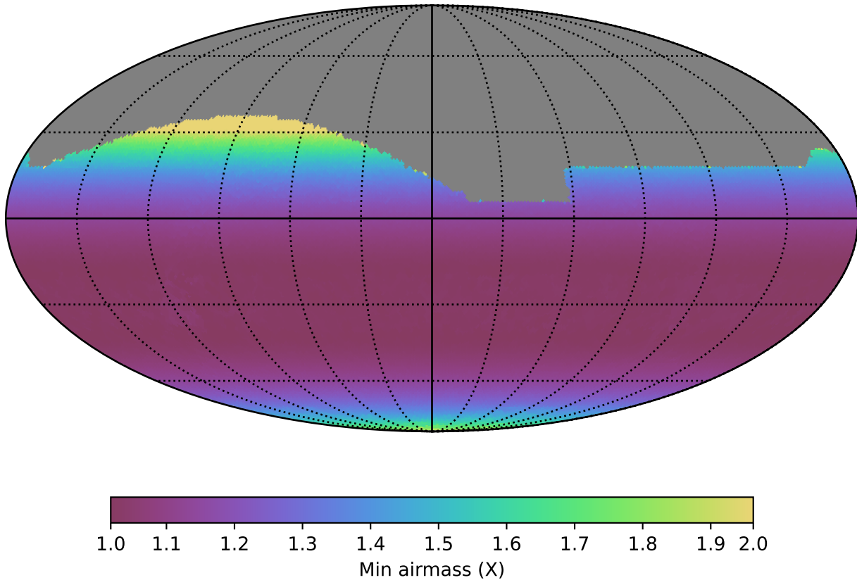
weather_cloudso1v3.4_10yrs All sky i band: Min airmass
