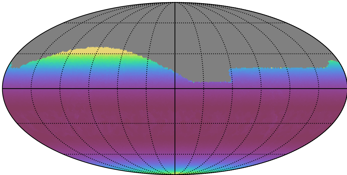
weather_cloudso1v3.4_10yrs All sky g band: Min airmass
