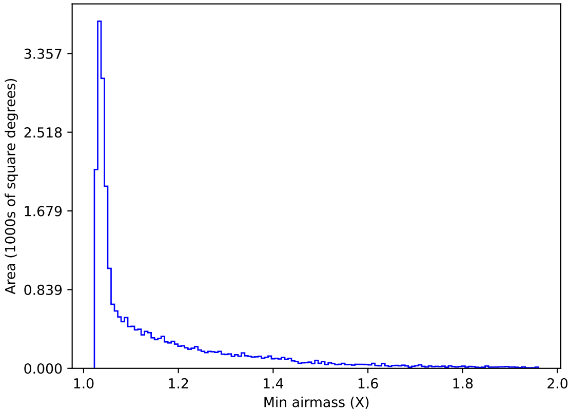
weather_cloudso1v3.4_10yrs All sky g band: Min airmass
