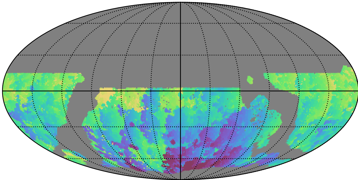
weather_cloudso1v3.4_10yrs WFD u band: Min HA
