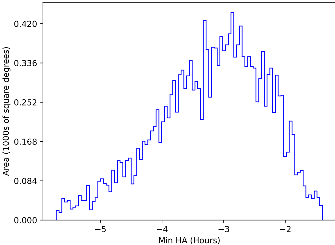
weather_cloudso1v3.4_10yrs WFD u band: Min HA
