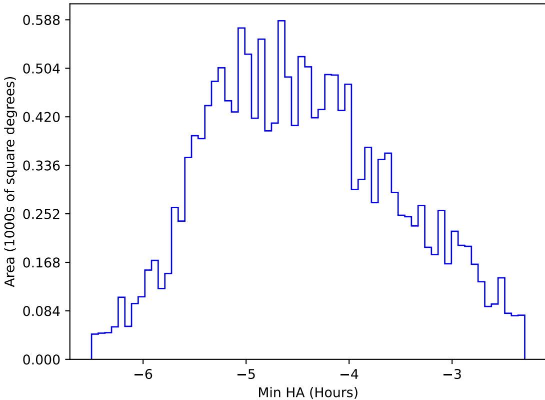
weather_cloudso1v3.4_10yrs WFD r band: Min HA
