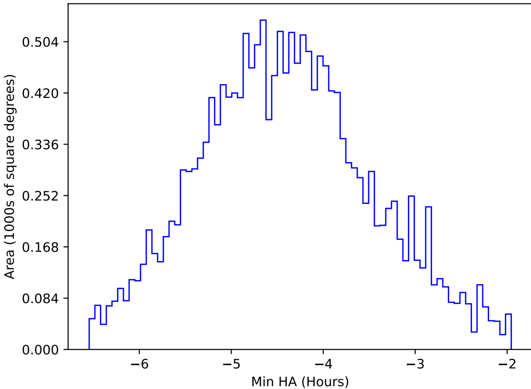
weather_cloudso1v3.4_10yrs WFD i band: Min HA
