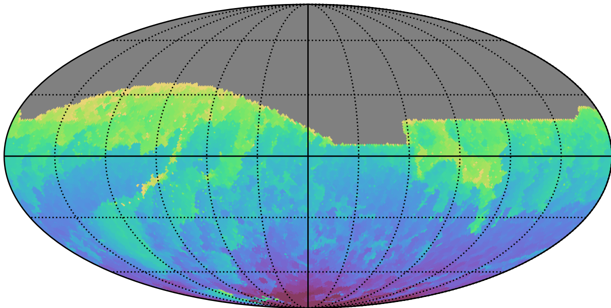
weather_cloudso1v3.4_10yrs All sky z band: Min HA
