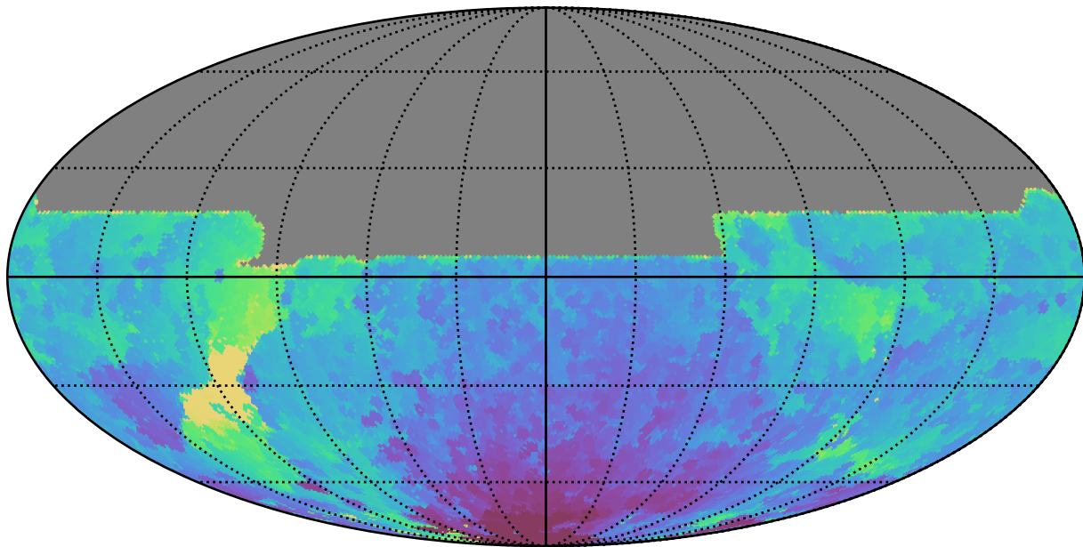
weather_cloudso1v3.4_10yrs All sky y band: Min HA
