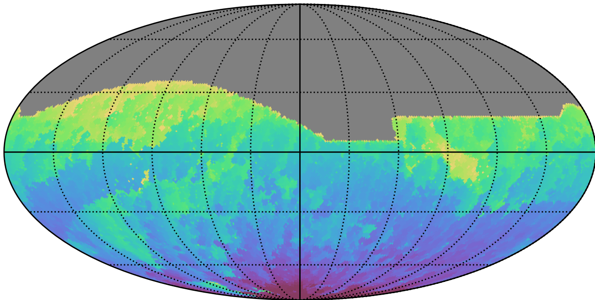
weather_cloudso1v3.4_10yrs All sky i band: Min HA
