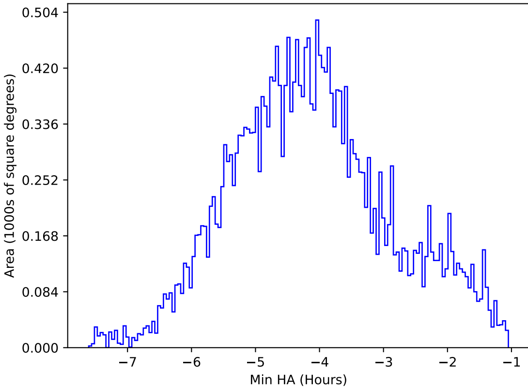
weather_cloudso1v3.4_10yrs All sky i band: Min HA
