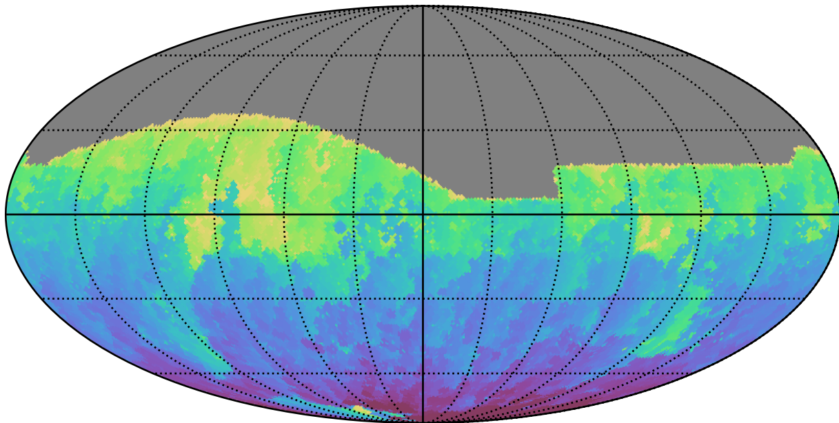
weather_cloudso1v3.4_10yrs All sky g band: Min HA
