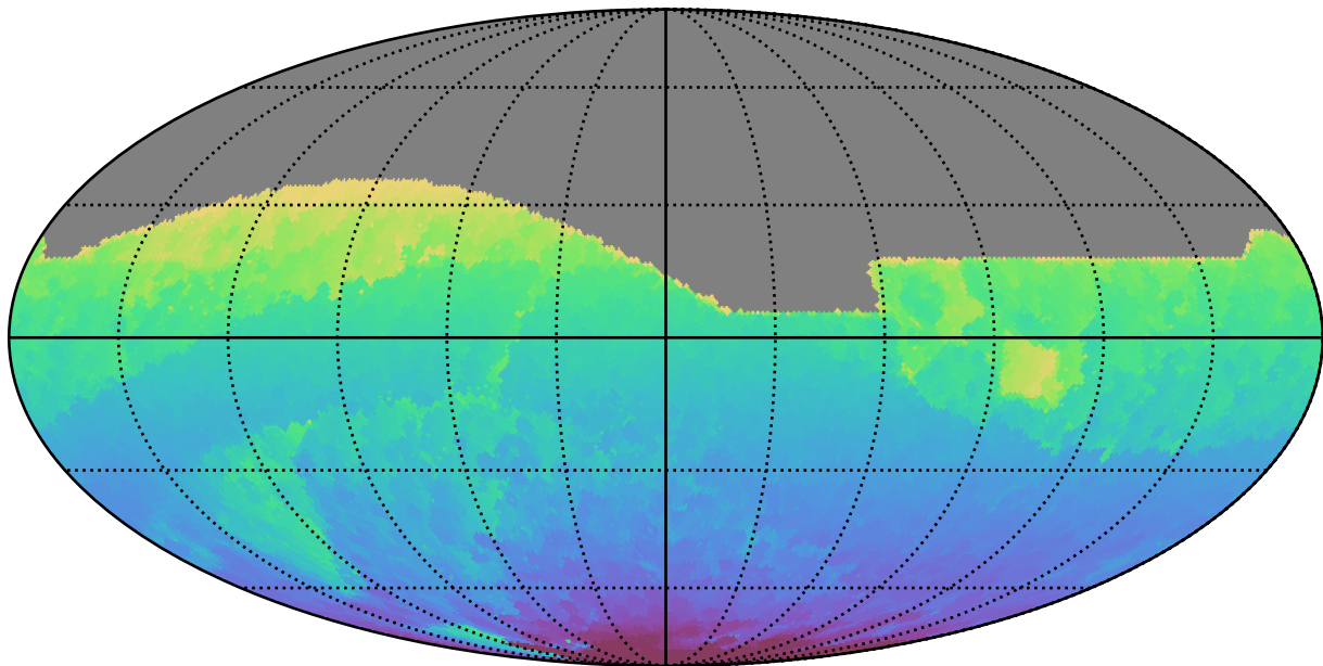
weather_cloudso1v3.4_10yrs All sky all bands: Min HA
