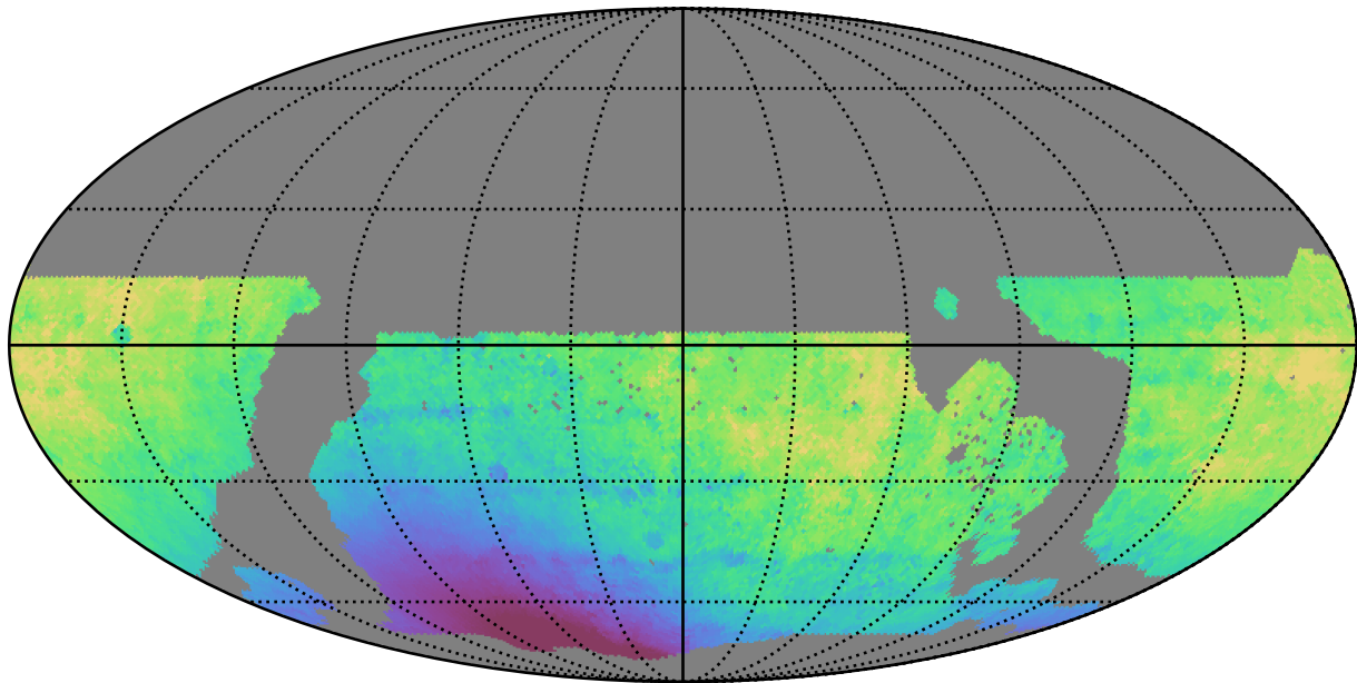
weather_cloudso1v3.4_10yrs WFD z band: Median solarElong
