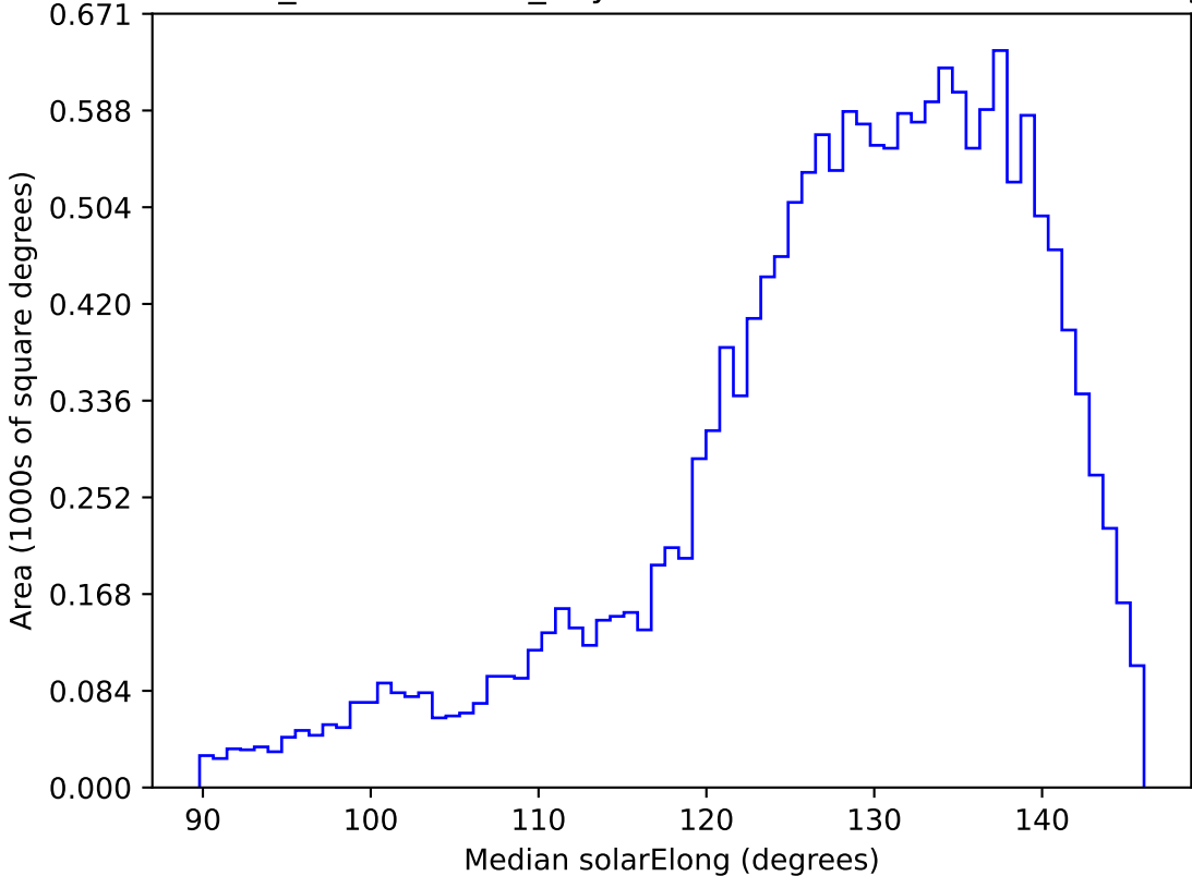
weather_cloudso1v3.4_10yrs WFD z band: Median solarElong
