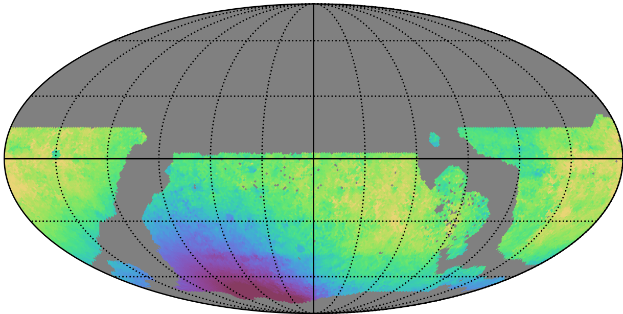
weather_cloudso1v3.4_10yrs WFD y band: Median solarElong
