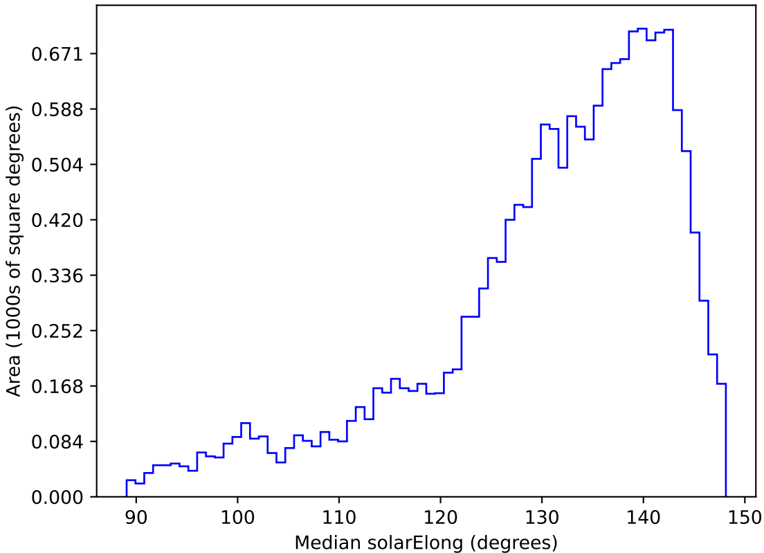
weather_cloudso1v3.4_10yrs WFD y band: Median solarElong
