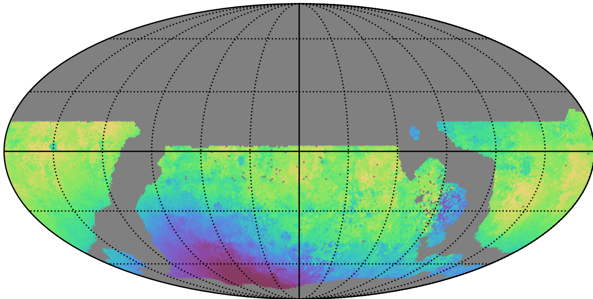
weather_cloudso1v3.4_10yrs WFD u band: Median solarElong
