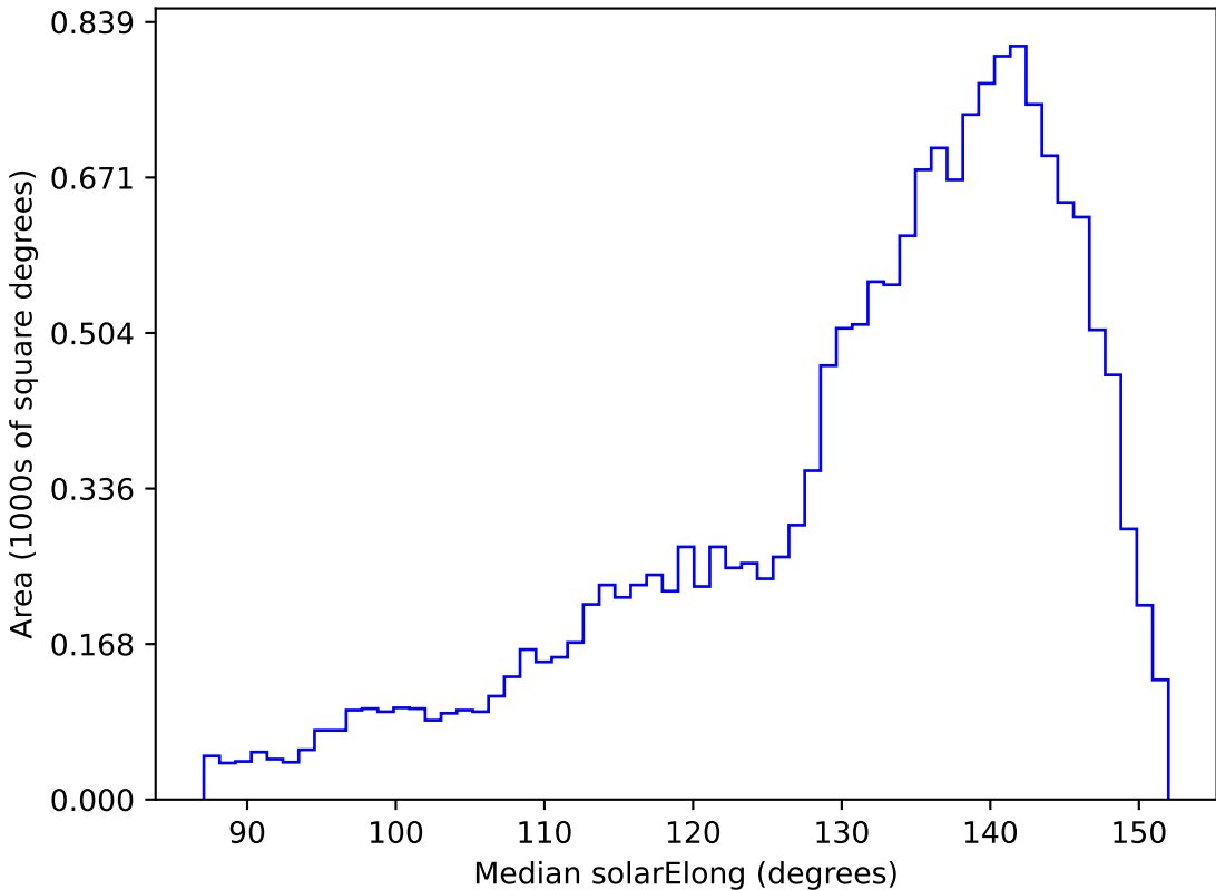
weather_cloudso1v3.4_10yrs WFD u band: Median solarElong
