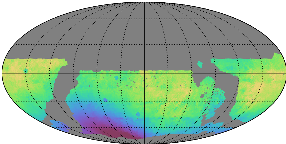
weather_cloudso1v3.4_10yrs WFD r band: Median solarElong
