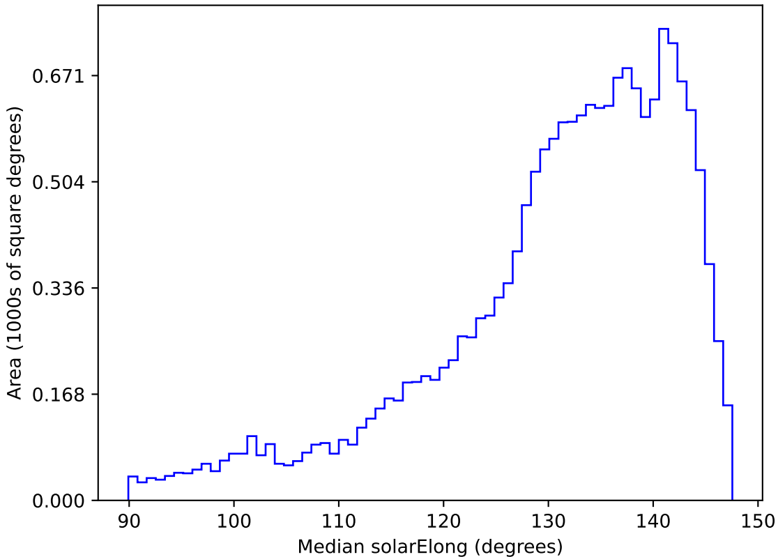
weather_cloudso1v3.4_10yrs WFD r band: Median solarElong
