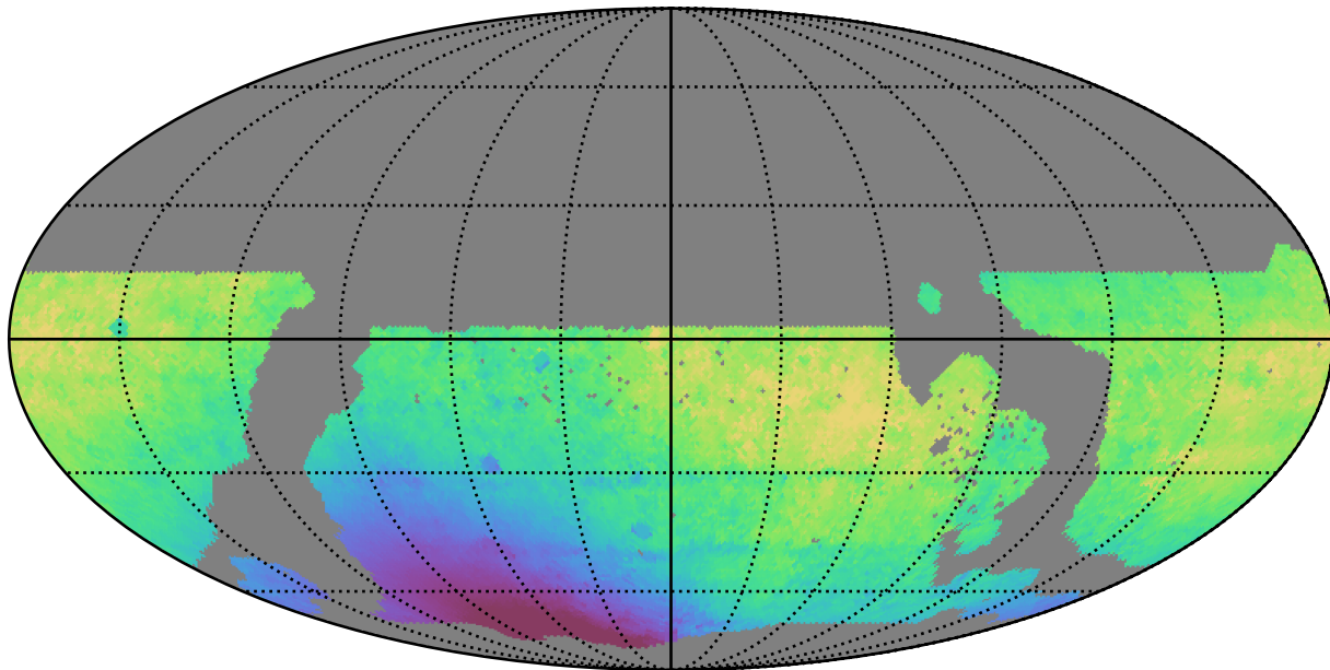
weather_cloudso1v3.4_10yrs WFD i band: Median solarElong
