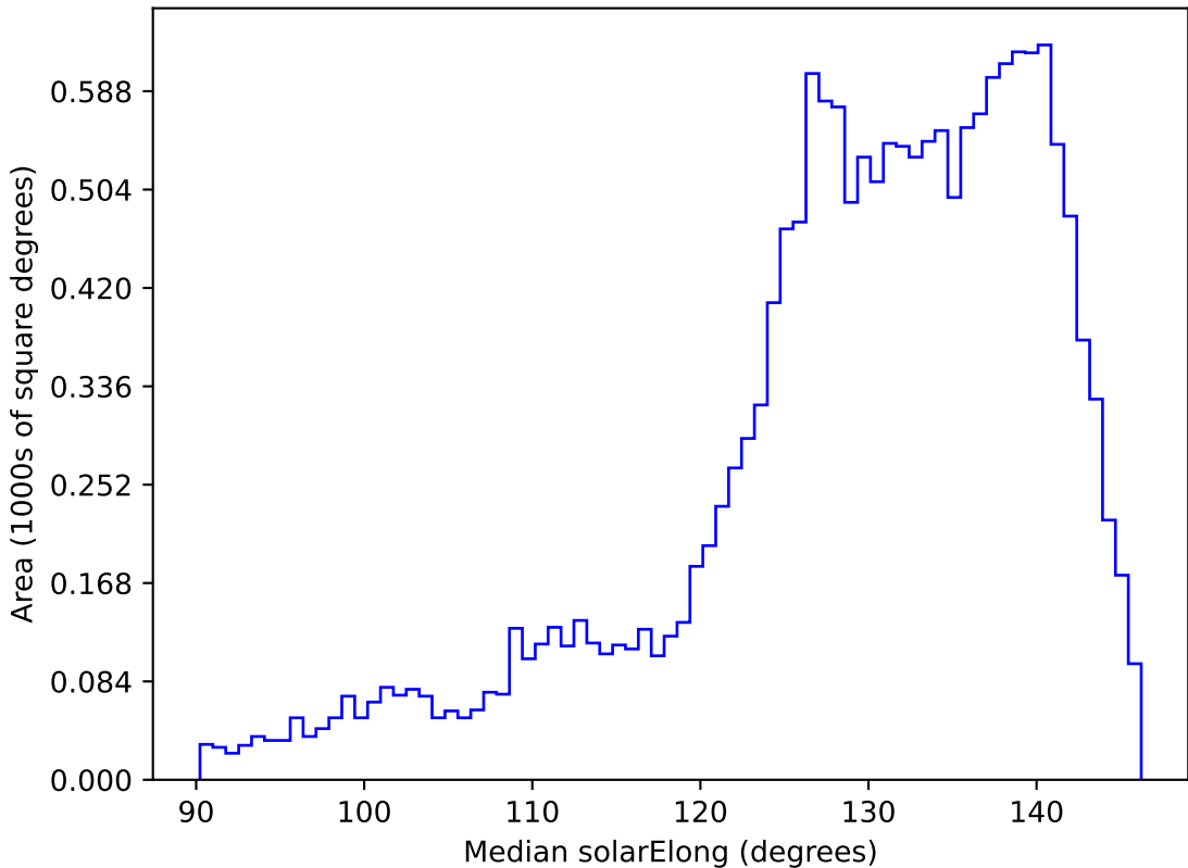
weather_cloudso1v3.4_10yrs WFD i band: Median solarElong
