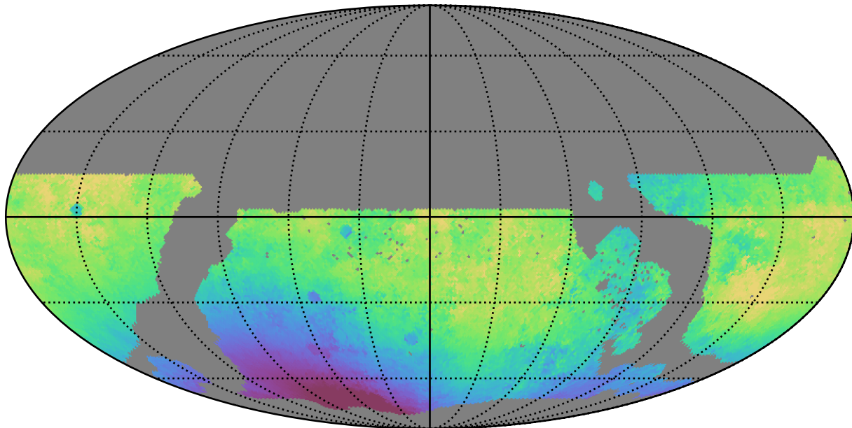
weather_cloudso1v3.4_10yrs WFD g band: Median solarElong
