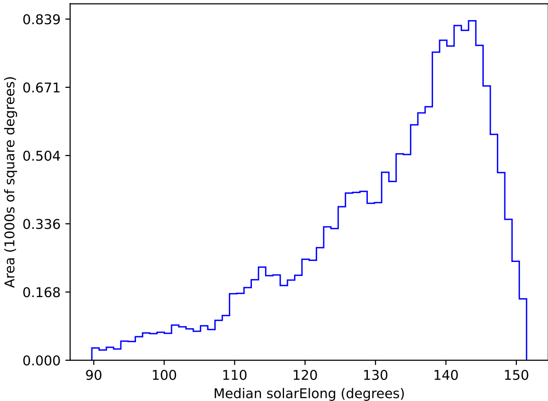
weather_cloudso1v3.4_10yrs WFD g band: Median solarElong
