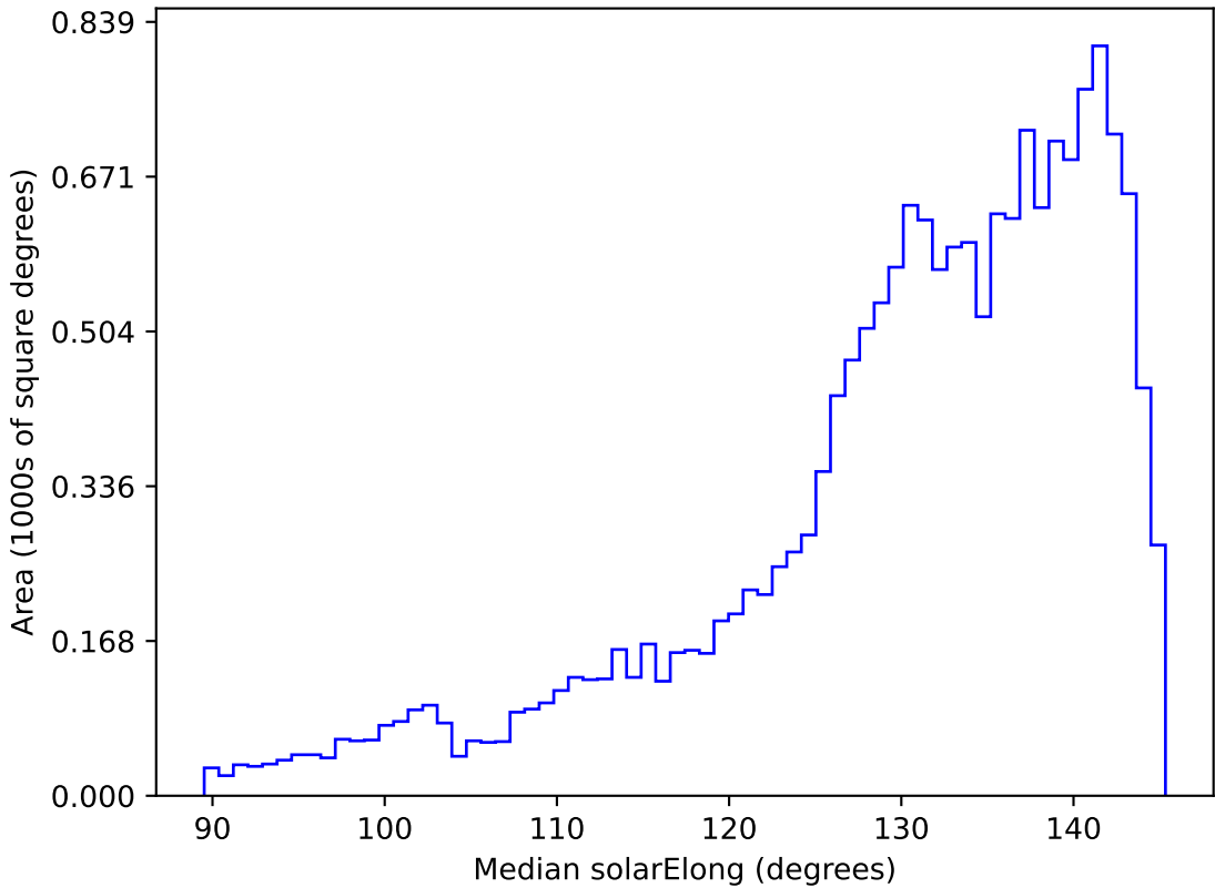
weather_cloudso1v3.4_10yrs WFD all bands: Median solarElong
